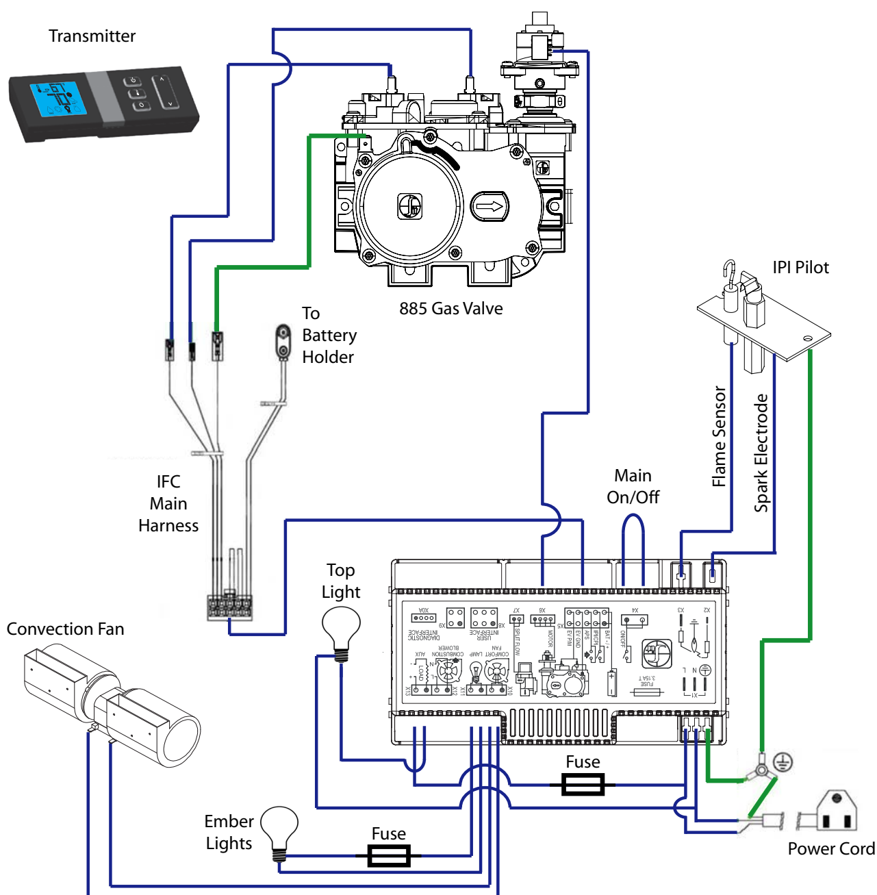
Figure 78: Proflame 2 Wiring Diagram
