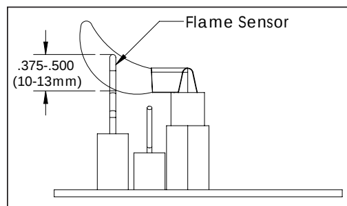
Figure 17. Pilot Light
